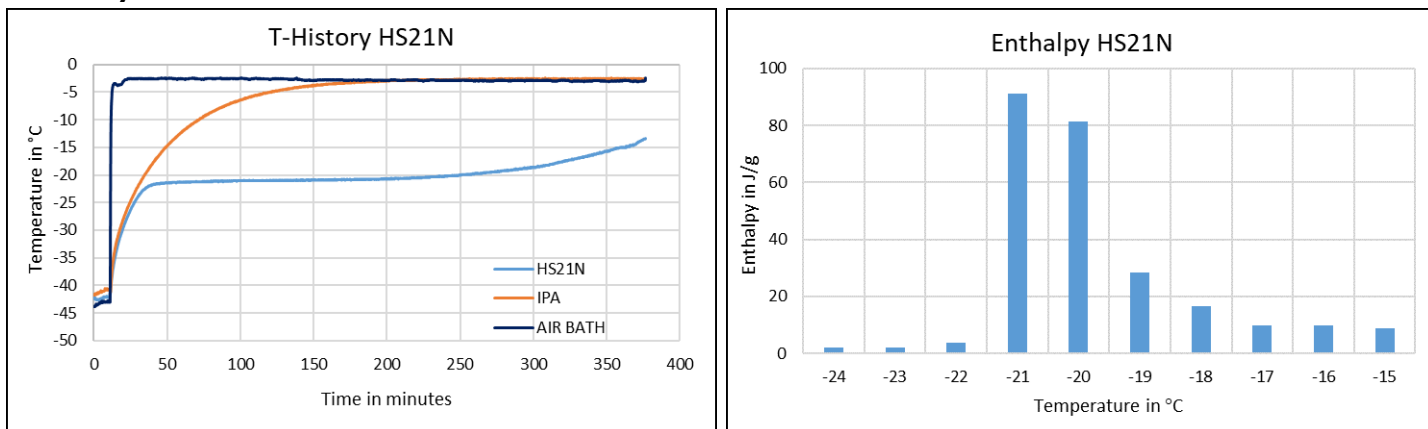
Fig1: T-History and Enthalpy profile of HS21N done in air bath
